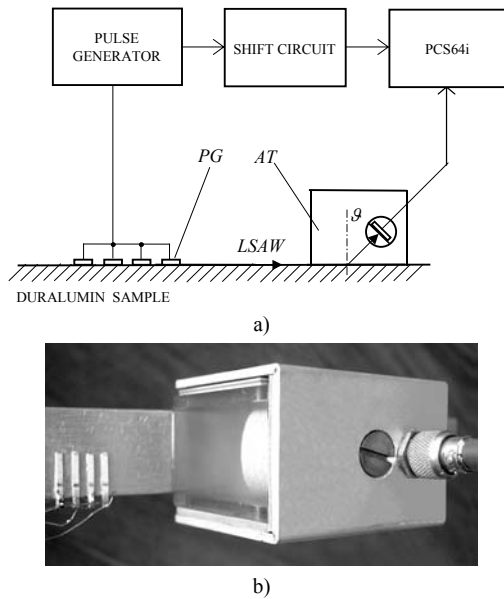
Fig.7. Piezoelectric grating investigation scheme (a) and top view of piezoelectric grating together with the angular transducer (b). PG is the piezoelectric grating, AT is the angular transducer
