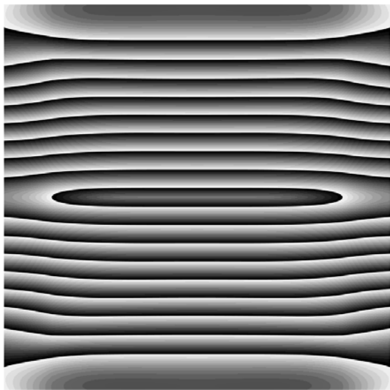
Fig.8. The equivalent stress represented by intensity mapping with smoothing
