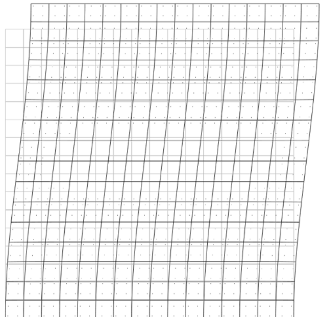
Fig. 7. The mesh in the status of equilibrium (shown in gray) and the statically distorted mesh in the cavalier projection with the points of numerical integration in the plastic region
