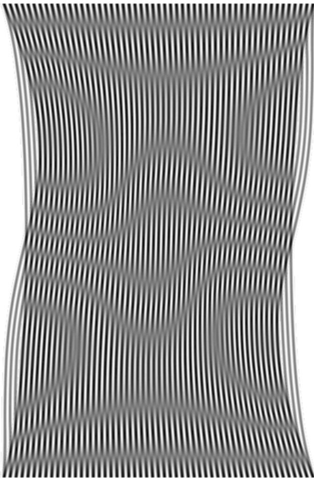
Fig. 5. The stroboscopic moire fringes for the seventh eigenmode
