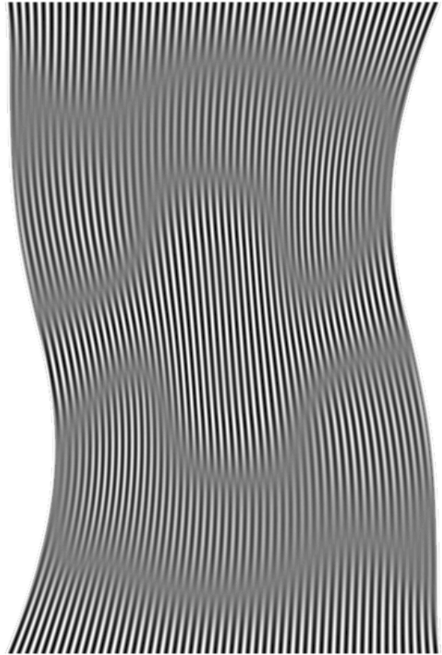
Fig. 6. The moire fringes obtained as a superposition of the linear system and the one taking the nonlinearity into account for the second eigenmode
