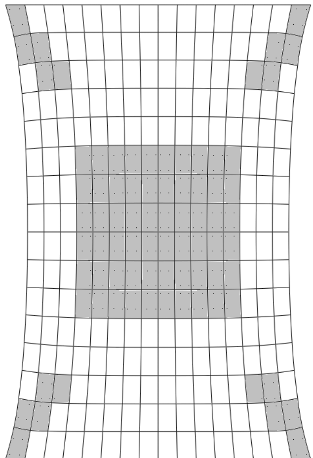
Fig.1. The statically distorted mesh with the points of numerical integration in the plastic region
