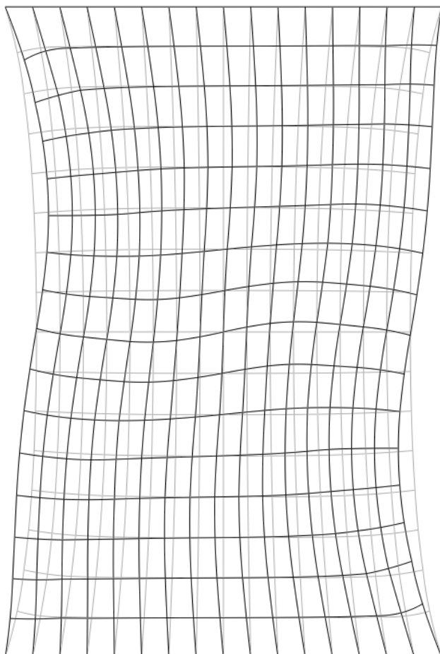
Fig. 2. The fifth eigenmode (the statically distorted mesh is gray while the eigenmode is black)
