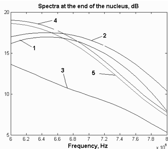
Fig.4. Spectra S_{PN}(f) in the end of the analyzed lens, there power spectra numbers from 1 to 5 corresponds to the signals in Fig.2
