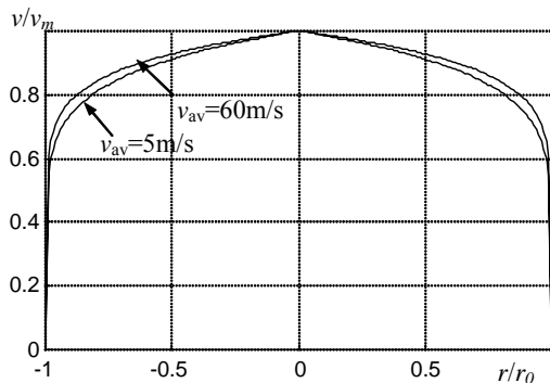
Fig.3. The distribution of normalized air flow velocity in the pipeline of 0.4m in diameter when the averaged flow velocity v_{av} = 5 m/s and 60 m/s
