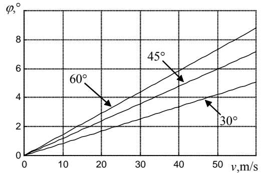
Fig.2. The dependence of the additional angle \varphi of deflection of transducers with respect the gas flow velocity when the flow sounding angle \alpha is changed
