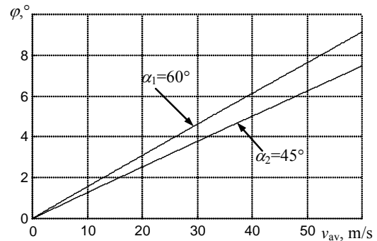
Fig. 4. The dependence of the additional angles of turn of the directivity patterns of transducers on the flow velocity when the angles of flow sounding \alpha_1 = 60^\circ and \alpha_2 = 45^\circ
