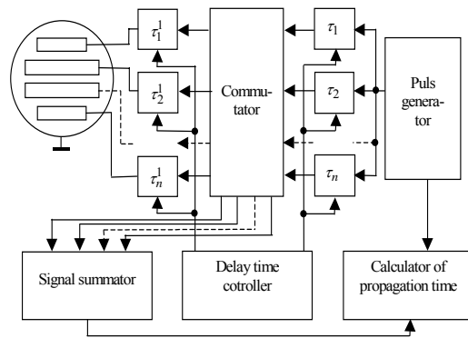
Fig. 5. Block diagram of equipment for control of directivity patterns
