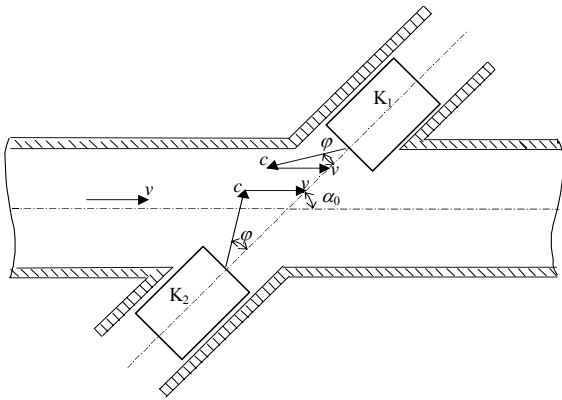
Fig. 1. The model of measuring channel with the deflected directional patterns of electroacoustical transducers
