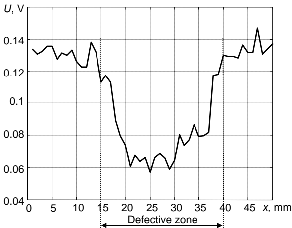
Fig.20. B – scan of the defective zone using through transmission testing technique
