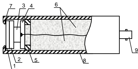
Fig. 1. Schematic drawing of the air – coupled transducer structure: 1, 2 – front face matching layers; 3 – piezoelement of the transducer; 4 – back matching layer; 5 – metallic ring; 6 – high – loss back material; 7 – glue; 8 – housing of the transducer; 9 – connector
