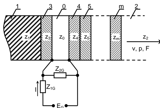
Fig. 2. Model of ultrasonic transducer. 0 – piezoelement, 1 - damper, 2 – surrounding media, 3 – back matching layer, 4, 5...m – front matching layers, E_G – electric voltage, I – current, Z_{1G} , Z_{2G} – electrical impedances
