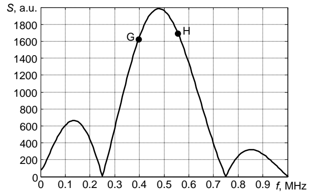
Fig.11. Spectrum of excitation signal; a.u. – arbitrary units
