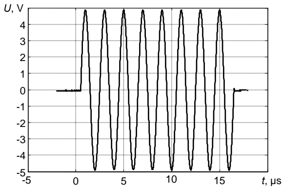
Fig.14. Time diagram of 8 periods excitation signal
