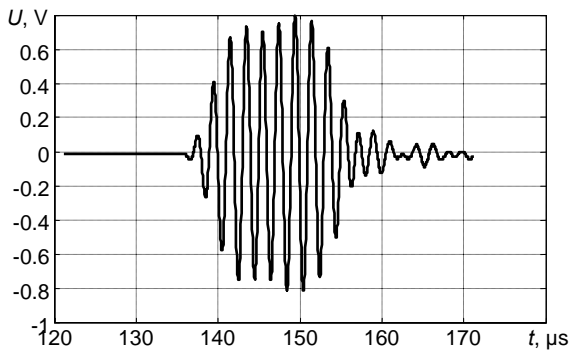
Fig.16. Signal at the output of the amplifier when the distance between transducers 50 mm.
