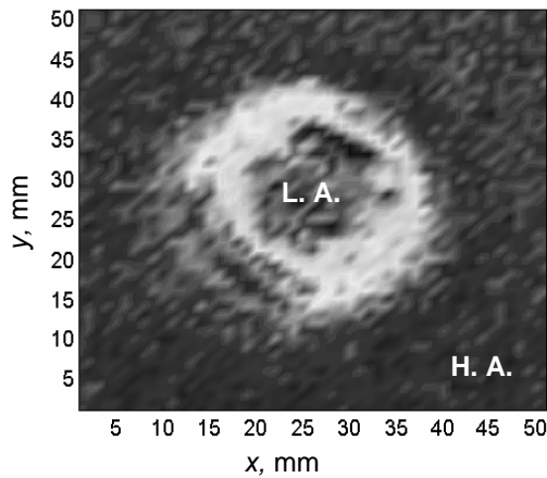
Fig.19. C - scan of the area with 25 mm defect carried out in the through transmission mode. (L.A. – low amplitude zone, H.A. – high amplitude zone)
