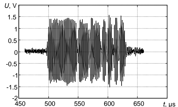
Fig.26. Received ultrasonic signal when the flow velocity 8.5m/s
