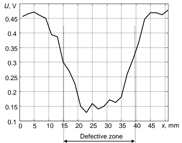
Fig.22. B – scan of the defective zone using through transmission testing technique with Lamb waves
