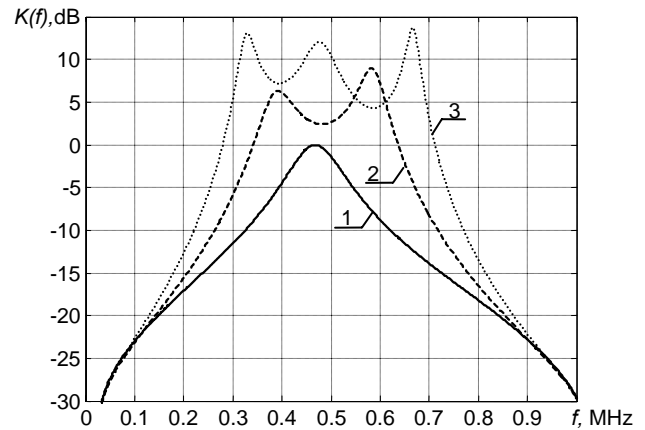
Fig. 3. Calculated transfer functions of the air – coupled ultrasonic transducer. 1 – transfer function of damped transducer without matching layers, 2 – transfer function of damped transducer with single \lambda/4 front matching layer, 3 - transfer function of damped transducer with double \lambda/4 front matching layer
