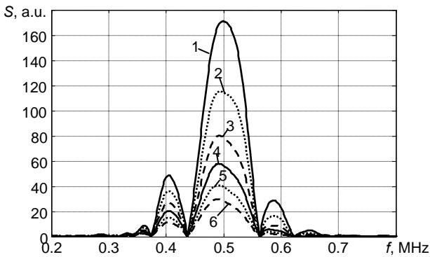
Fig.17. Dependence of a spectrum of the signal vs. distance between transducers. Distances between transducers: 1- 50mm, 2 – 100mm, 3 – 150mm, 4 – 200mm, 5 – 250mm, 6 – 300mm.
