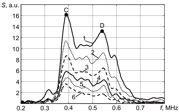
Fig.9. Dependence of a spectrum of the signal vs. distance between transducers. Distances between transducers: 1- 50mm, 2 – 100mm, 3 – 150mm, 4 – 200mm, 5 – 250mm, 6 – 300mm.
