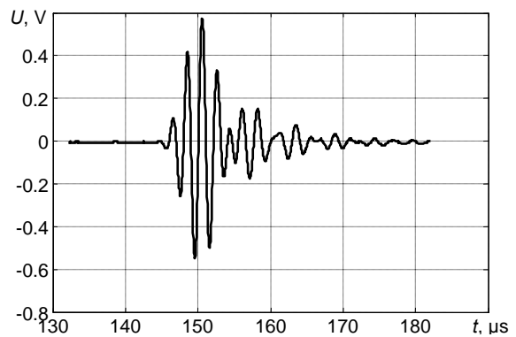
Fig.12. Signal on an output of the amplifier when distance between transducers 50mm
