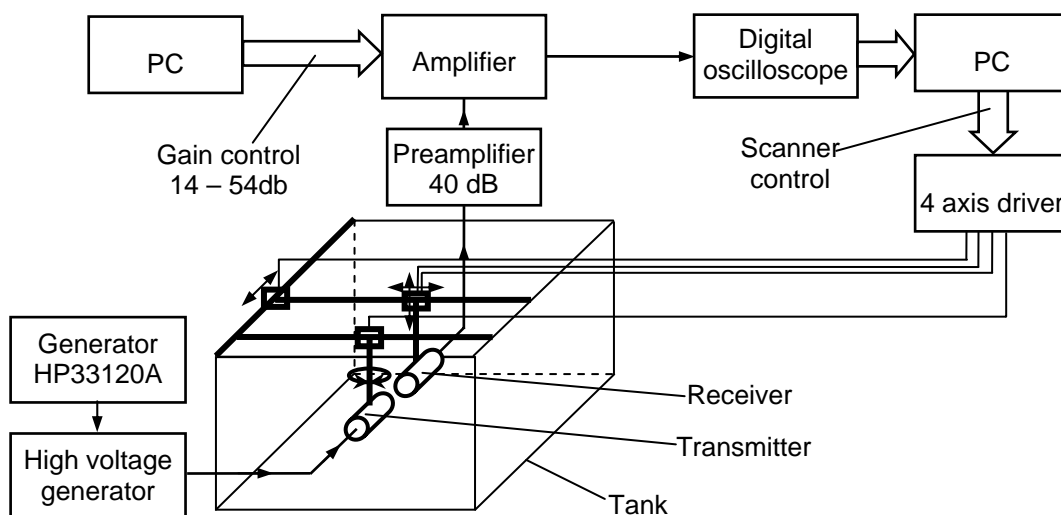
Fig.5. Block diagram of the experimental system
