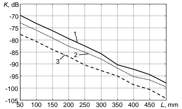
Fig.18. Transmission losses of air – coupled ultrasonic transducers vs. distance between the transducers when duration of the excitation pulse is 1 – 8 periods, 2 – 2 periods, 3 – 0.5 periods.
