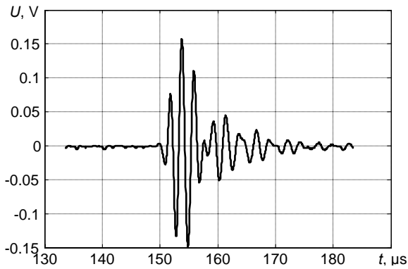
Fig.8. Signal on an output of the amplifier when distance between transducers 50mm. Duration of excitation signal – 0.5 period.
