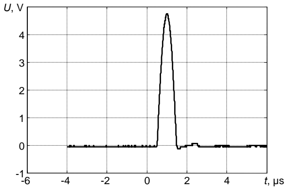
Fig.6. Time diagram of 0.5 period excitation signal
