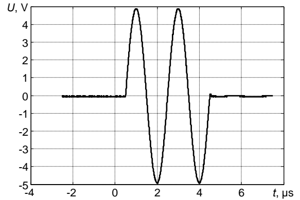
Fig.10. Time diagram of 2 periods excitation signal
