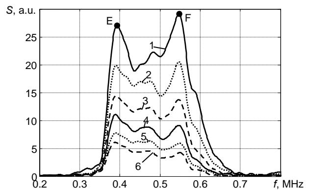
Fig.13. Dependence of a spectrum of the signal vs. distance between transducers. Distances between transducers: 1- 50mm, 2 – 100mm, 3 – 150mm, 4 – 200mm, 5 – 250mm, 6 – 300mm.
