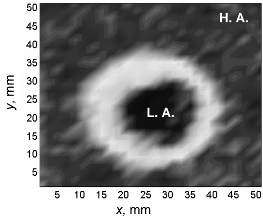
Fig.21. C - scan of the area with 25 mm defect carried out in the through transmission mode using a_0 Lamb wave. (L.A. – low amplitude zone, H.A. – high amplitude zone)
