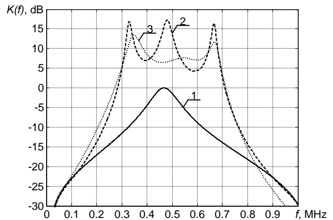
Fig. 4. Calculated transfer functions of the air – coupled ultrasonic transducer. 1 – transfer function of damped transducer without matching layers, 2 – transfer function of damped transducer with double \lambda/4 front and single \lambda/4 back matching layers, 3 - transfer function of damped transducer with double \lambda/4 and single \lambda/4 back matching layers and electrical matching circuit.
