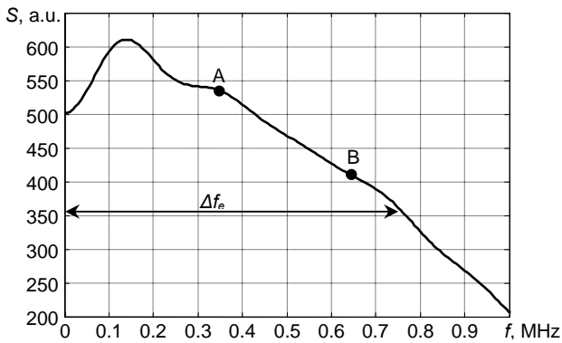
Fig.7. Spectrum of excitation signal; a.u. – arbitrary units
