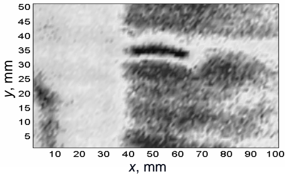
Fig. 24. The amplitude C – scan in one – side access mode with a_0 Lamb wave of the samples with impact defects: (a) – 1J impact defect,
