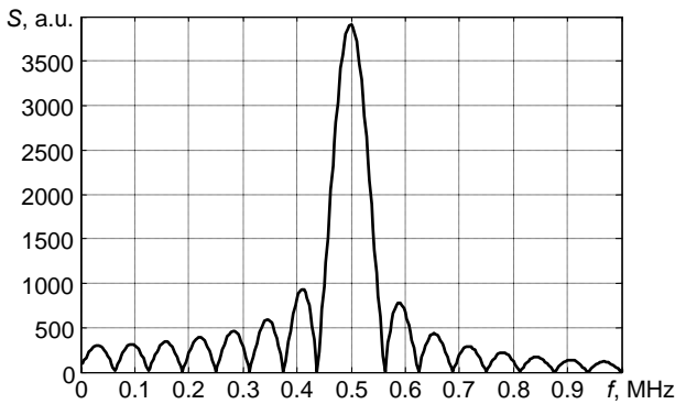
Fig.15. Spectrum of excitation signal; a.u. – arbitrary units
