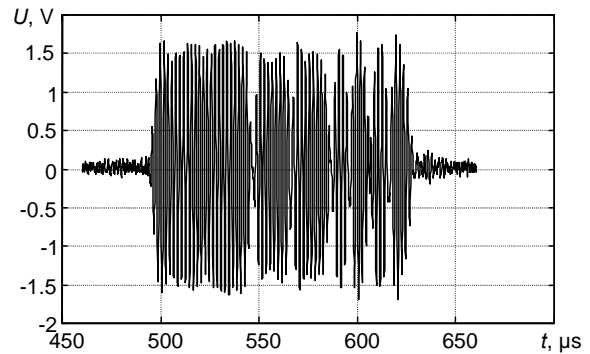
Fig.25. Received ultrasonic signal when the flow velocity 4.5m/s
