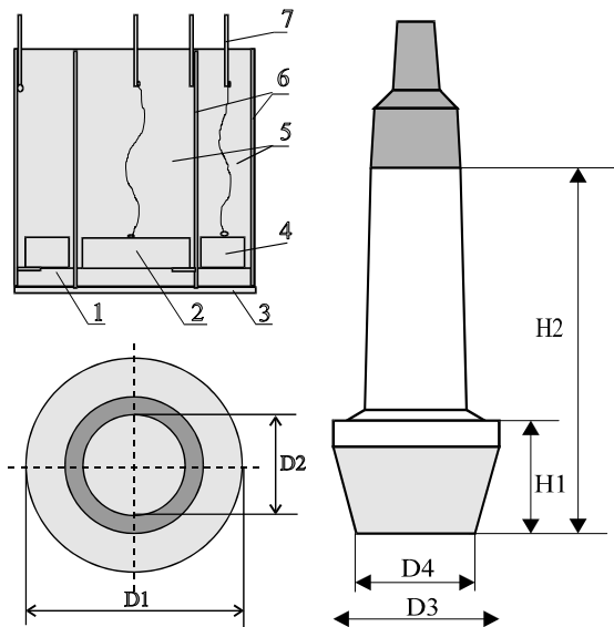
Fig. 3. Design of disc-ring Doppler transducer: 1-maching layer, 2-disc type piezoelectric crystal, 3-protector layer, 4-ring type piezoelectric crystal, 5-backing without damping layer, 6-insulating screen, 7-electrodes
