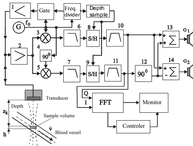
Fig.8. Main functional modules of the pulse-wave Doppler instrument
